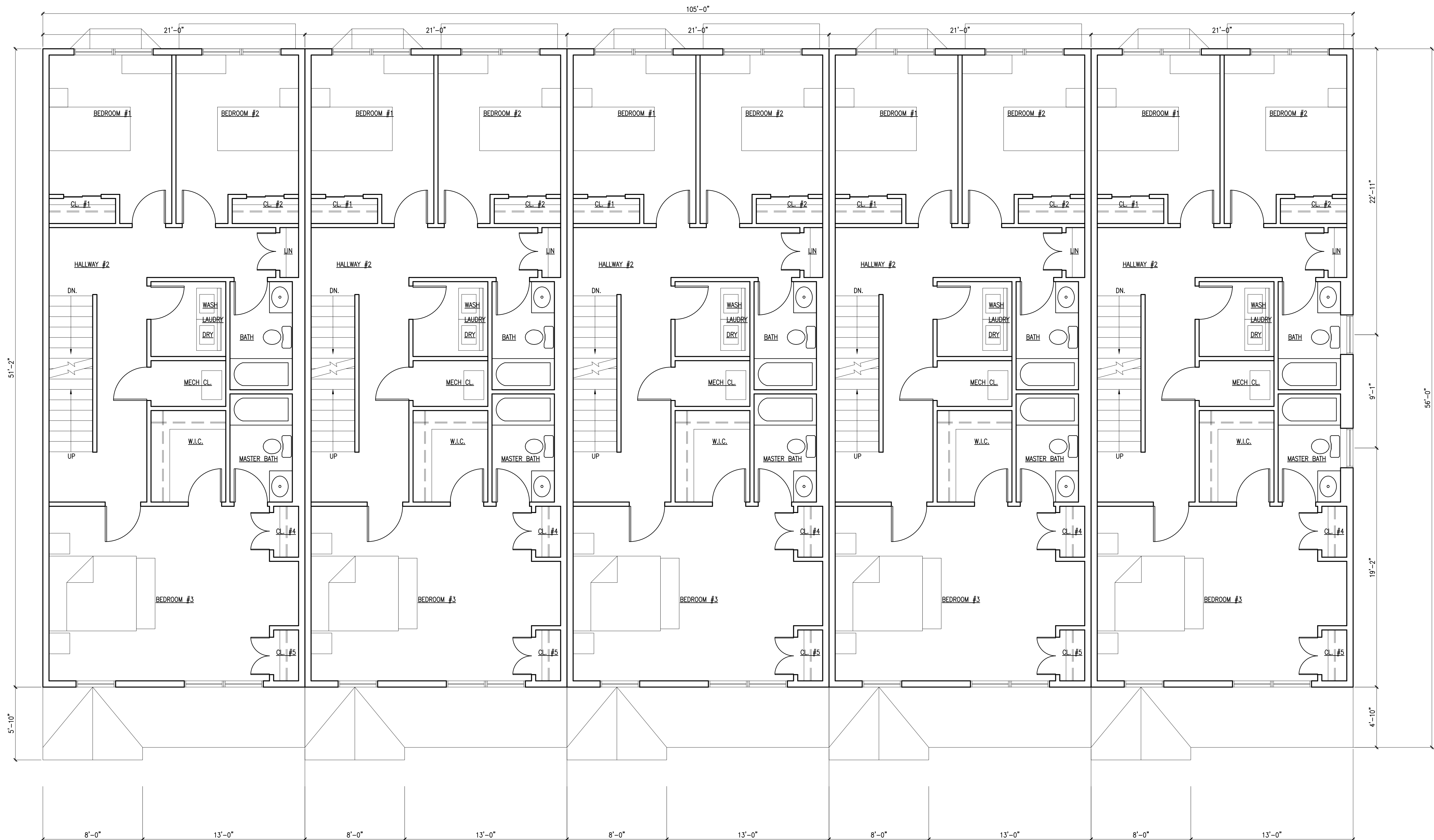
2ND. FL. SCALE: 1/4"=1'-0"
